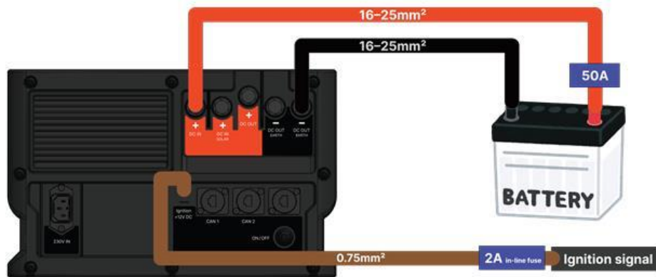
Figure 1 DC Charging for electrical vehicles
